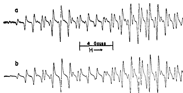
Figure 6. (a) First derivative esr spectrum of the anion radical produced by electroreduction of a 0.54 mM solution of 5 in DMF. The low-field half of the spectrum is shown. (b) Computed spectrum using a_N = 9.71 , a_H = 3.395 and 1.02 , a_P = 11.06 gauss, and 0.125-gauss line width.
