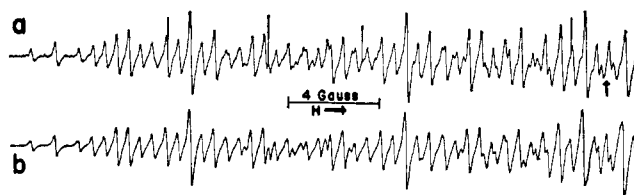
Figure 4. (a) First derivative esr spectrum of the anion radical produced by electroreduction of a 0.46 mM solution of 3 in DMF. Slightly more than the low-field half of the spectrum is shown. The center of the spectrum is indicated by the arrow. (b) Computed spectrum using a_N = 9.70 , a_H = 3.34 , 1.08 , and 2.79 , a_P = 17.60 gauss, and 0.140 -gauss line width.
